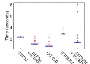
Fig. 9: AWS IoT connection establishment
