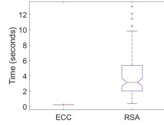
Fig. 7: ECC (256) and RSA (1024) keypair generation for the ESP32
