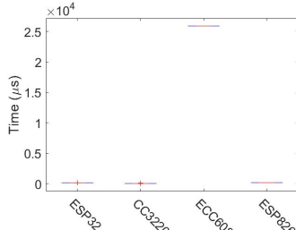
Fig. 5: HMAC with SHA-256
